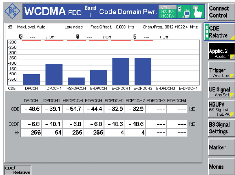
The “code domain error relative” application shows the results of the relative code domain error (CDE) and of the effective code domain power (ECDP) measurements for all active codes. The test covers the requirements defined in 3GPP TS 34.121/5.13.2 which request such figures in the presence of HSPA channels.
