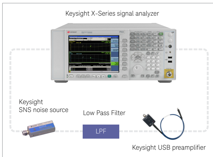
Figure 3. USB preamplifier calibration setup
