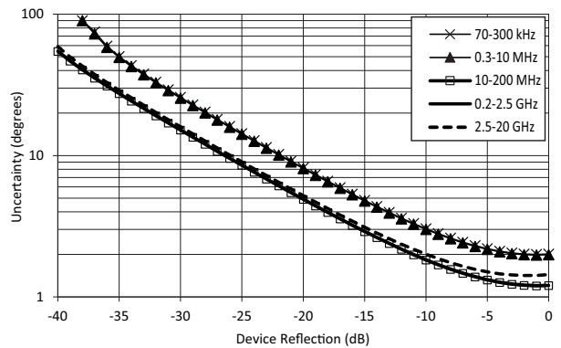
Reflection Phase Uncertainty; MS4642B (Opt. 61/62); SOLT Calibration using 3650A 3.5 mm Cal Kit
