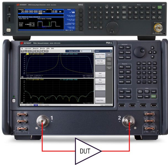
Classic NPR measurement with PNA-L and UXG
