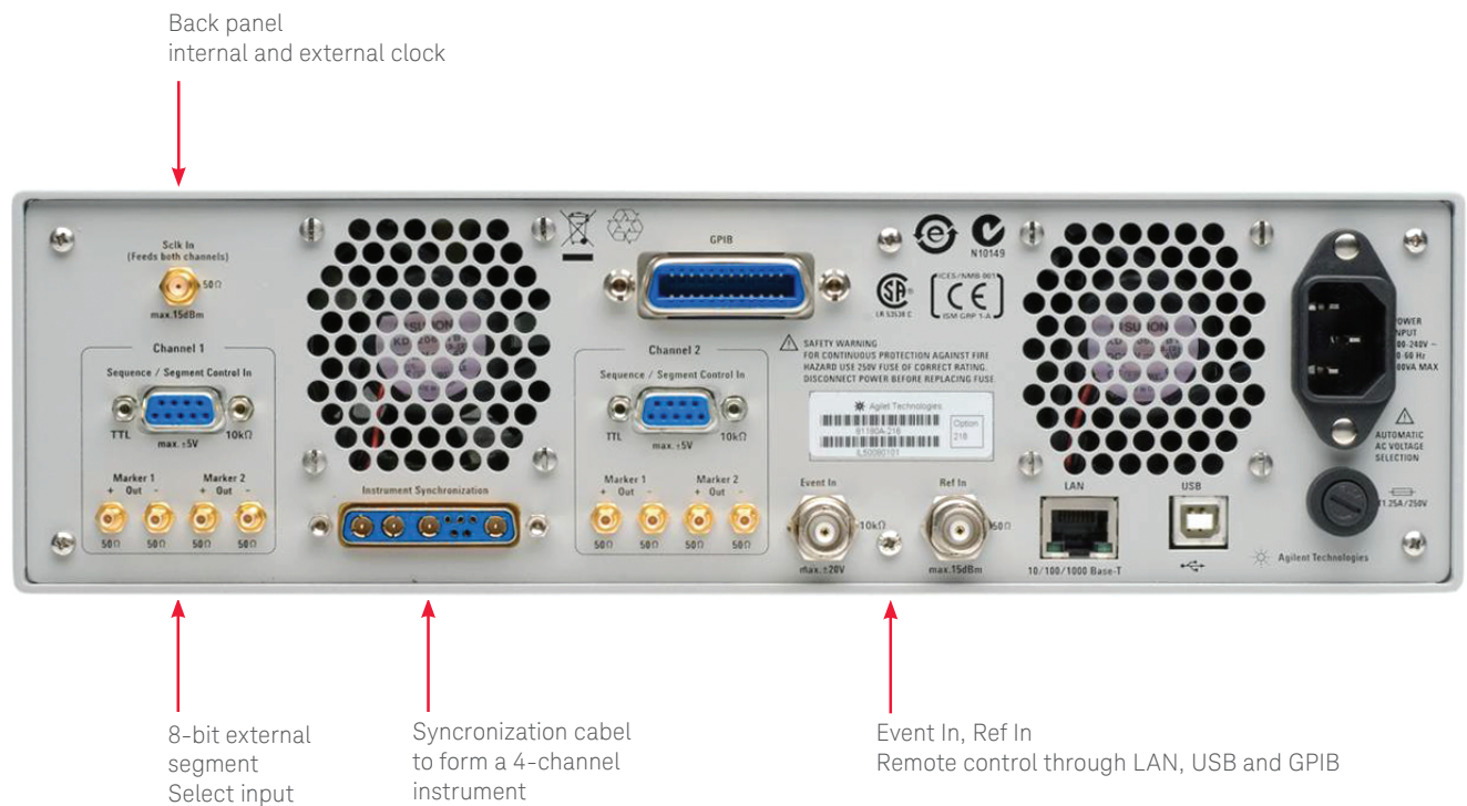
Figure 3. Back panel
