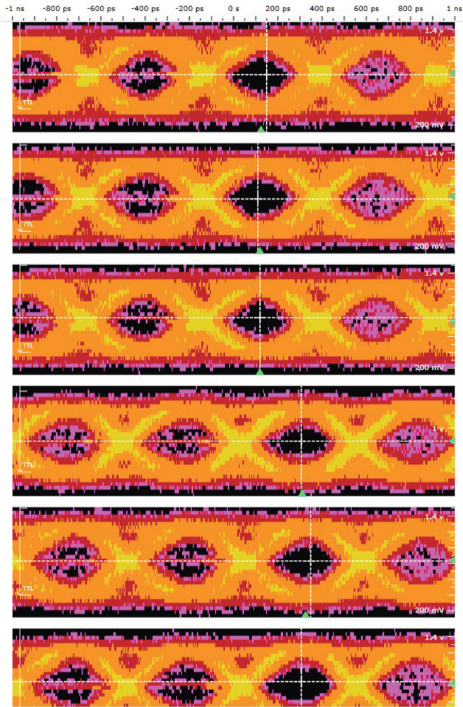
Figure 8. Eye scan clearly indicates the DDR3 byte lane shift caused by fly-by routing.
