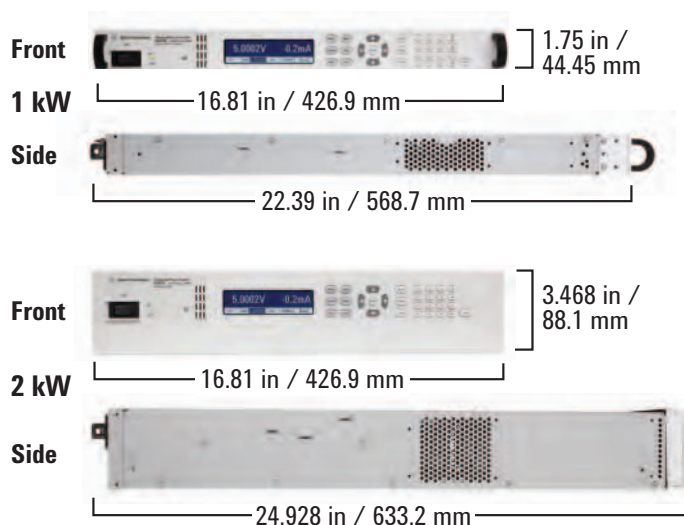
Figure 12. 1 kW and 2 kW power supplies, front and side dimensions
