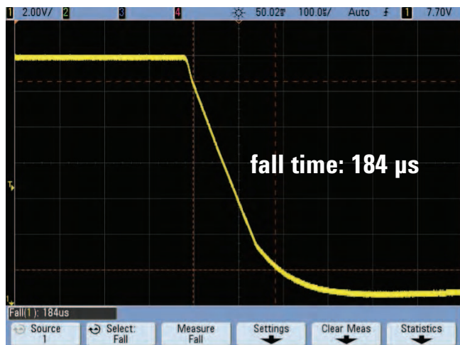
Figure 5. Interrupt pulse fall time measurement of < 200 us
