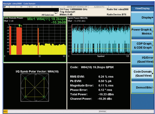
Figure 2. Code Domain Power quad view
