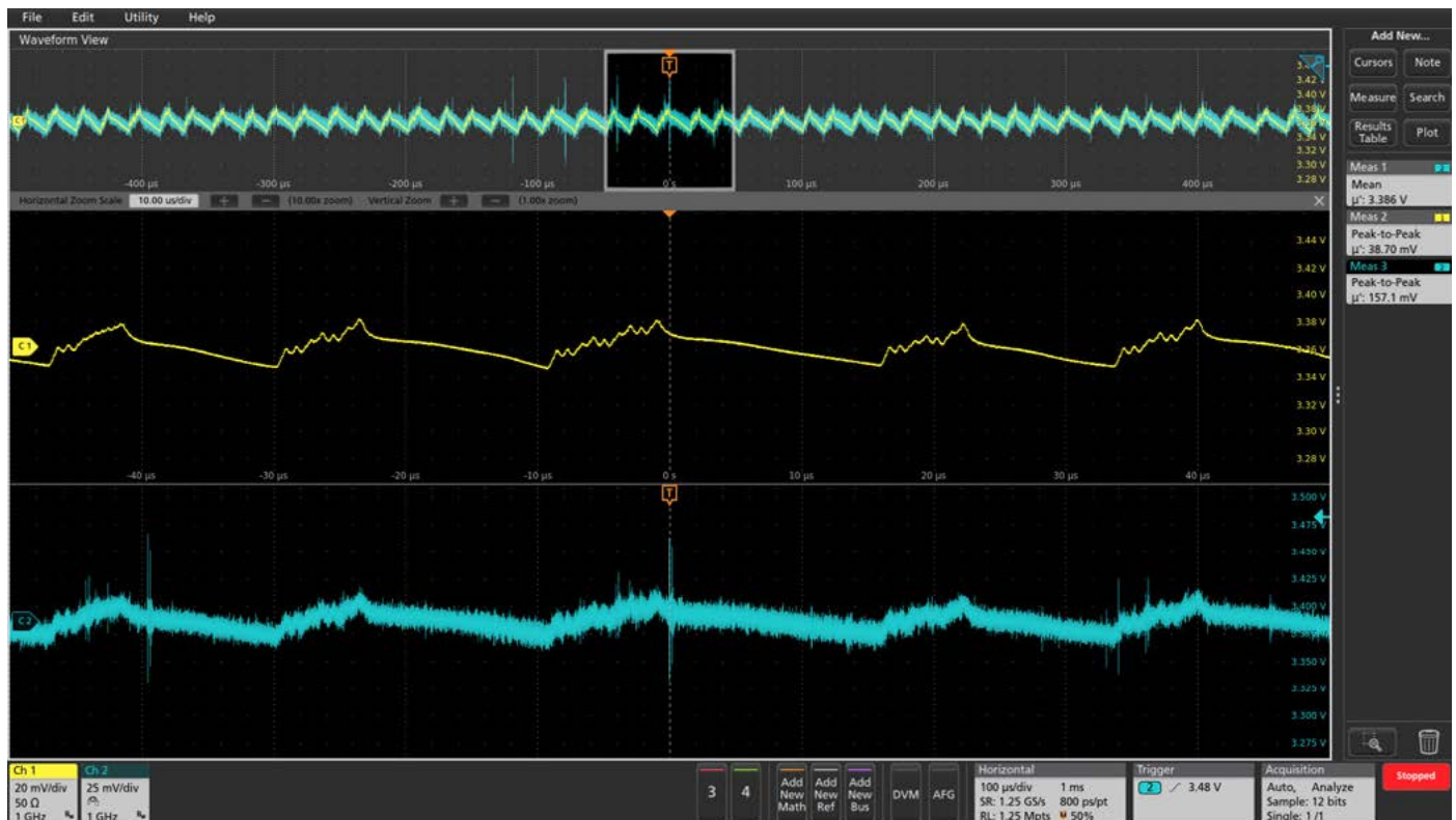
Figure 6. Channel 2 (blue trace) shows the 157.1 mV peak-to-peak noise of a traditional 10x passive probe compared to 38.7 mV peak-to-peak when using a Tektronix TPR1000 power rail probe on channel 1 (yellow trace).
