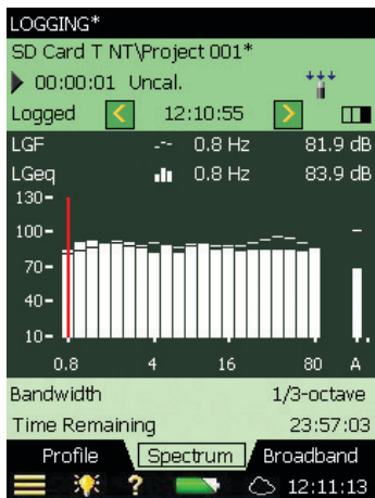
Fig. 13 Low Frequency Option showing G-weighted parameters L_{GF} and L_{Geq}
