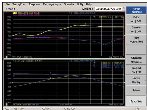
Application of power level control for amplifier gain compression at 98 GHz.
