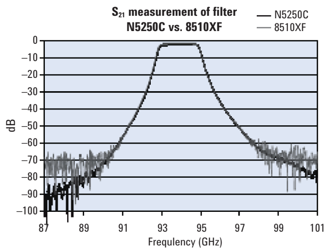
The N5250C PNA-based mmwave system has superb dynamic range. Shown here is the S_{21} of a filter at 94 GHz, compared to the 8510XF.
