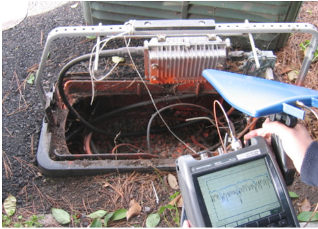
Figure 1a. FieldFox connected to a directional antenna for locating a source of radio interference
