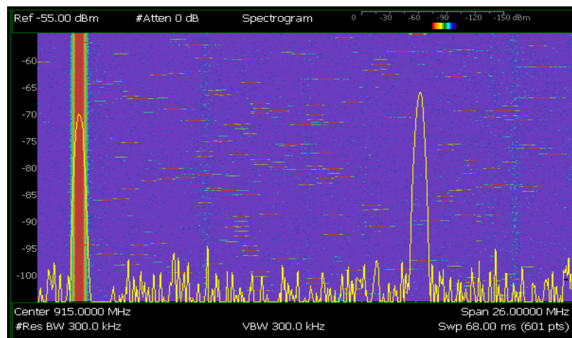
Figure 10. This shows a spectrogram display of a frequency hopping signal and a measurement sweep using the standard Clear/Write mode (yellow trace) superimposed over the spectrogram.
