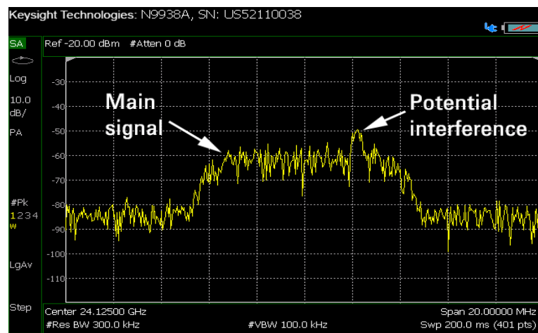
Figure 4. Measured spectrum of a 24 GHz microwave communications signal with lower-than-expected system performance and including potential in-band interference
