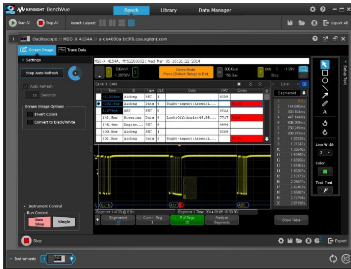
Figure 36. BV0004B BenchVue
