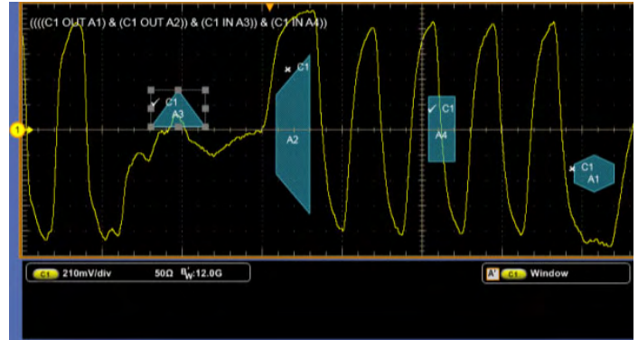
Visual Trigger finds unique events in complex waveforms.
