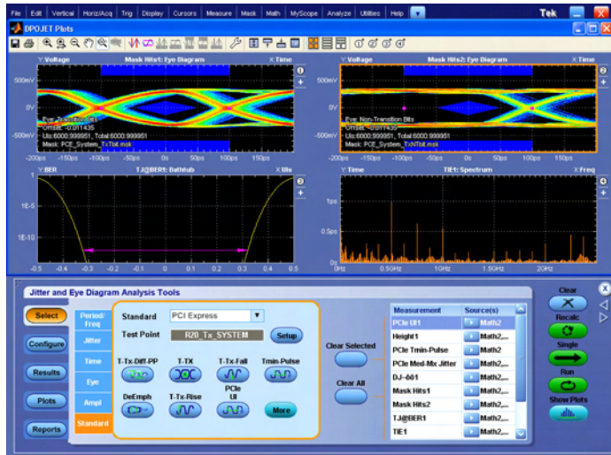
PCI Express Analysis Test Solution (Option PCE3) – Analyze the performance of your PCI Express Rev 1.0, 2.0, or 3.0 design with comprehensive test support. Using DPOJET, Option PCE3 enables tests that conform to PCI-SIG standards.
