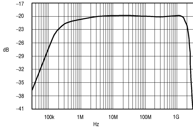
CT6 Typical Frequency Response.
