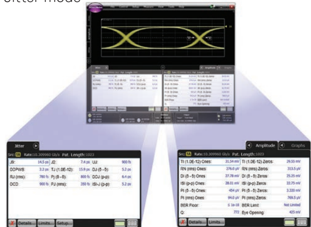
Precision jitter, amplitude, and frequency analysis capability
