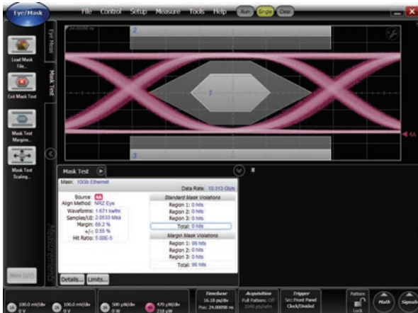
A digital communication analyzer providing fast transmitter characterization using eye diagram analysis, calibrated reference receivers, and automated mask margin measurements
