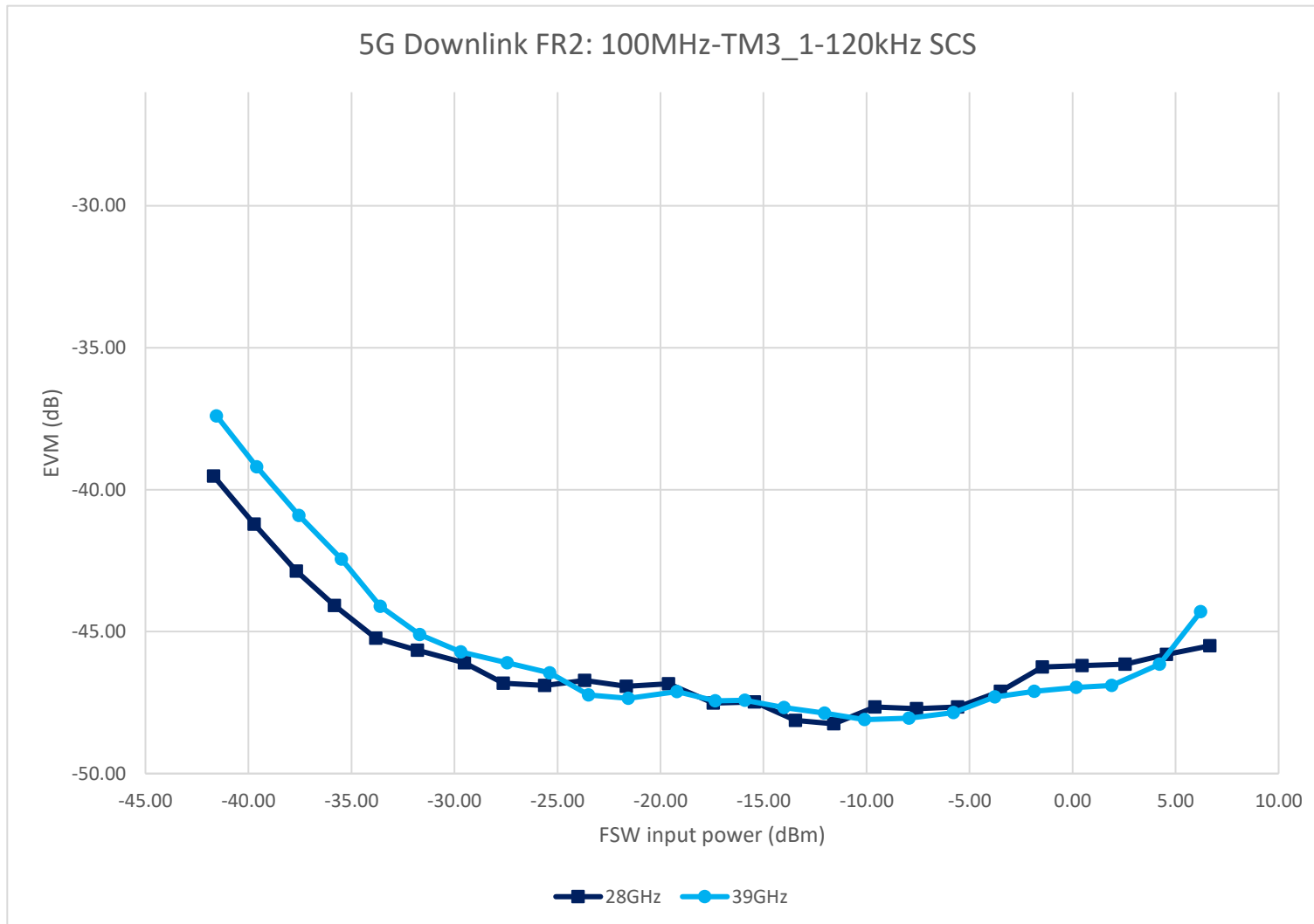
EVM (meas.) for different input power selections measured with the R&S®FSW50-B4001 12
