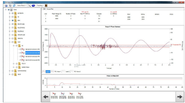
Surge test results with Partial Discharge (PD)
