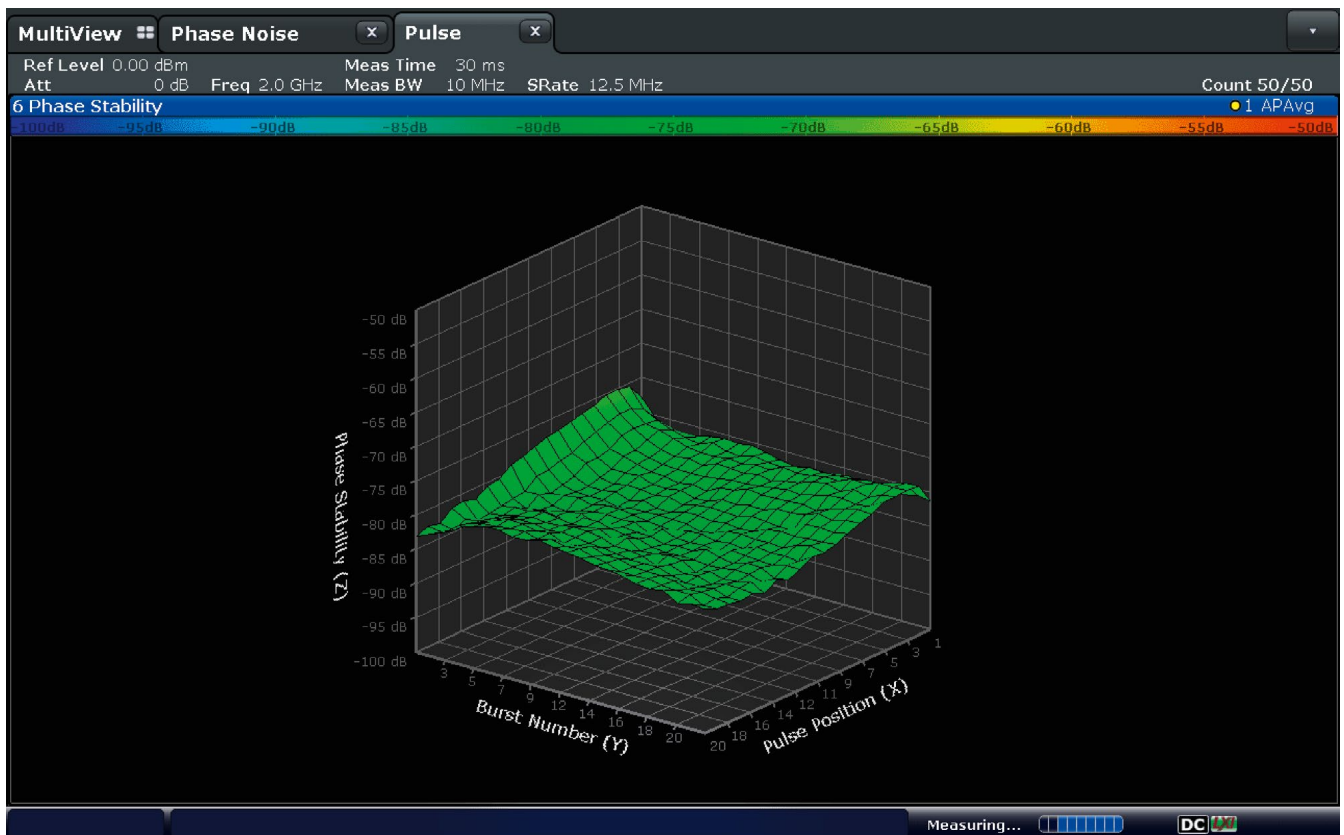
3D plot of the phase stability of pulses in various pulse sequences (bursts).
