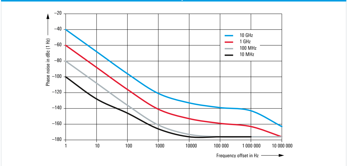
Phase noise of the internal local oscillator at various frequencies
