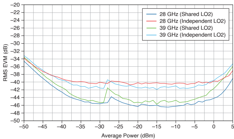
Figure 39. Direct TRX to Direct TRX RF 5G NR 1 CC × 100 MHz RMS EVM versus Average Power, Measured [27],[28]
