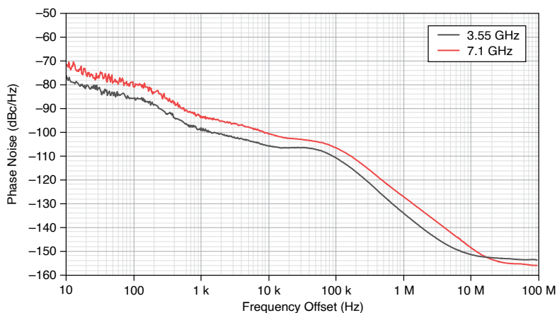
Figure 49. PXIe-3622 Internal LO1 VCO Phase Noise, Measured [37] (Spurs Not Shown)
