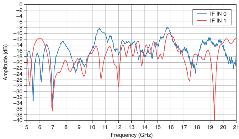
Figure 42. PXIe-3622 IF IN Port Return Loss, Measured
