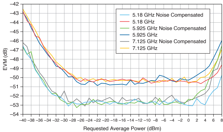
Figure 30. WLAN 802.11ax 80 MHz RMS EVM Versus Average Power, Measured [18],[19]
