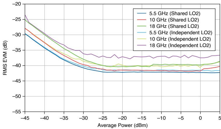
Figure 36. IF 5G NR 2 CC x 400 MHz RMS EVM versus Average Power, Measured [20],[24]
