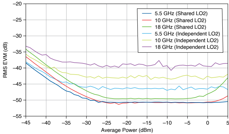
Figure 33. IF 5G NR 1 CC x 100 MHz RMS EVM versus Average Power, Measured [20],[21]
