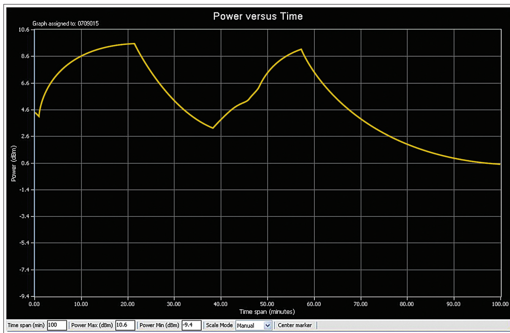
Power versus Time graph shows the effect of turning on and off the cooling fan of a 2 GHz power amplifier
