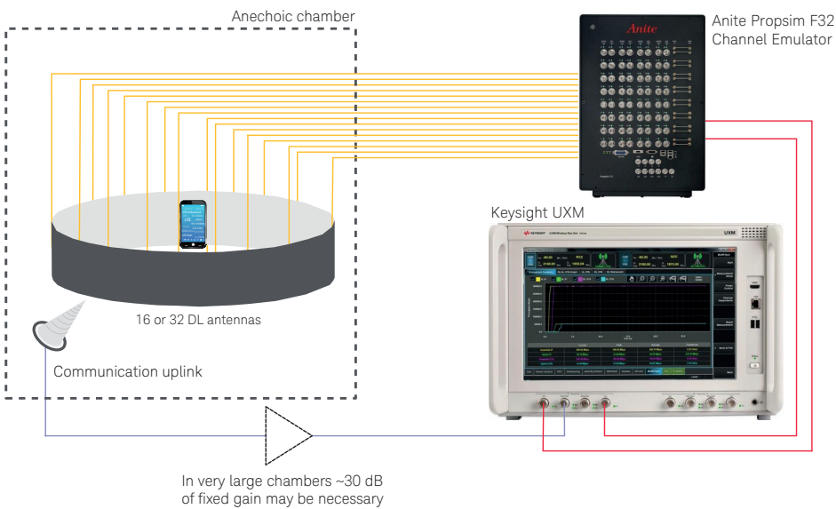
Figure 17. Typical multi-probe anechoic chamber MIMO OTA test system. (Note: Anite is now part of Keysight Technologies)
