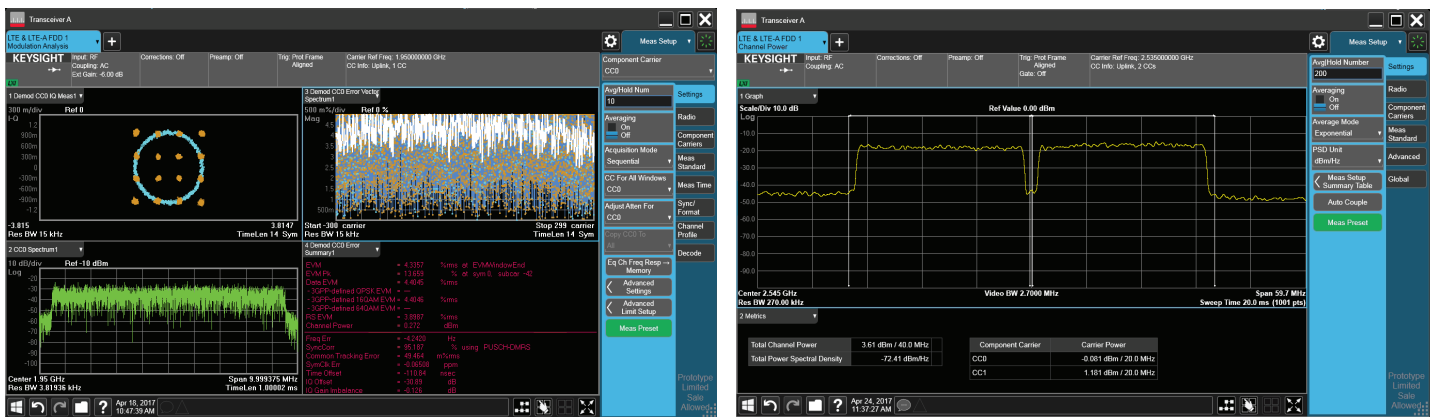
Figure 21. The UXM's built-in X-Series measurement applications provide consistent, repeatable transmitter testing
