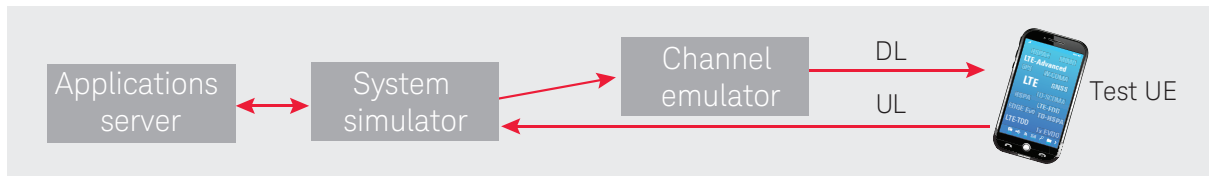
Figure 4. Realistic end-to-end data throughput testing is essential for today's wireless devices
