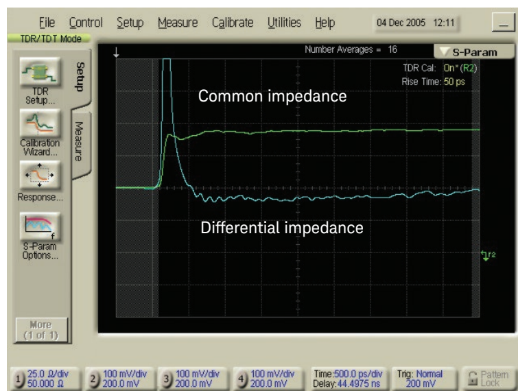
Figure 59. Measured reflected common signal from a coax to twisted pair transition with an incident common signal.
