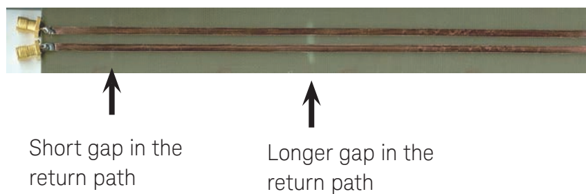
Figure 43. Tightly coupled pair of transmission lines with small gaps in the return path that will generate ground bounce.
