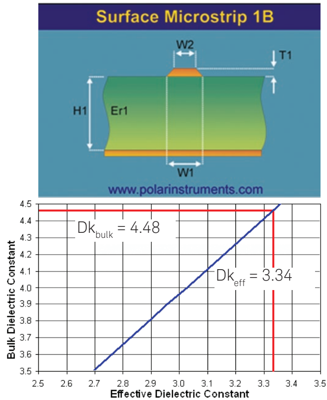
Figure 13. Using a field solver to back out the bulk dielectric constant from the effective dielectric constant.
