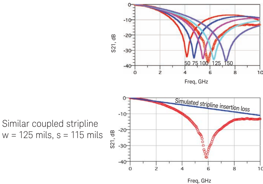
Figure 35. Changing separation between the two transmission lines showing the impact on the insertion loss dip.
