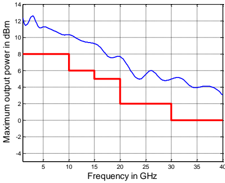
Maximum output power in dBm versus frequency of the R&S ® ZNB40, models .82 and .84
