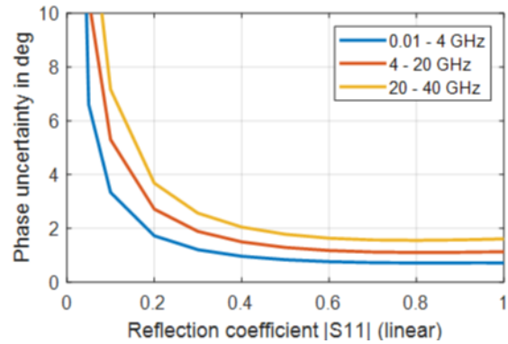
Uncertainty of reflection magnitude and reflection phase measurements of the R&S®ZNB40, model .72 in the frequency range from 10 MHz to 40 GHz; analysis conditions: S_{12} = S_{21} = 0 , cal. power -10 dBm, meas. power -10 dBm
