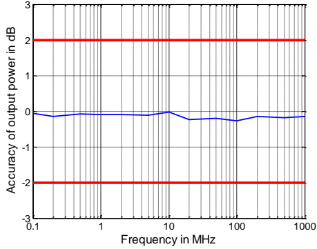
Output power accuracy in dB versus frequency of the R&S ® ZNB40, models .82 and .84
