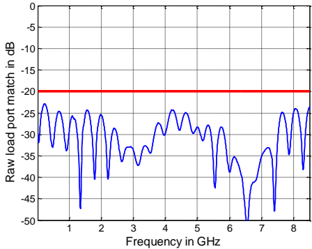
Raw load port match versus frequency of the R&S ® ZNB8 1
