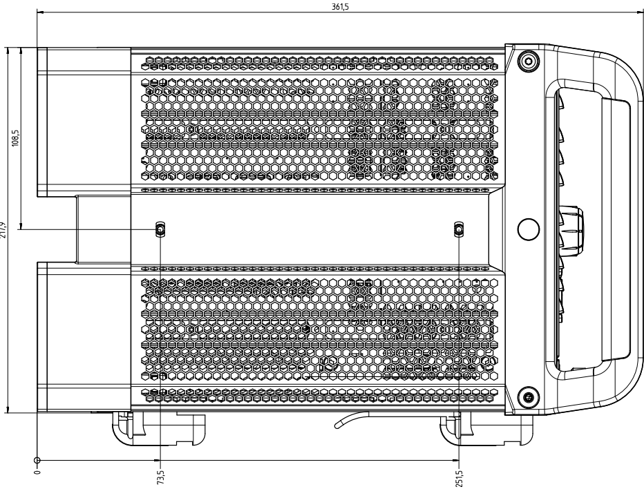
Side view of the R&S ® ZNB
