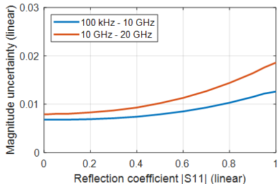
Uncertainty of reflection magnitude and reflection phase measurements of the R&S®ZNB20 1 in the frequency range from 100 kHz to 20 GHz; analysis conditions: S_{12} = S_{21} = 0 , cal. power -10 dBm, meas. power -10 dBm
