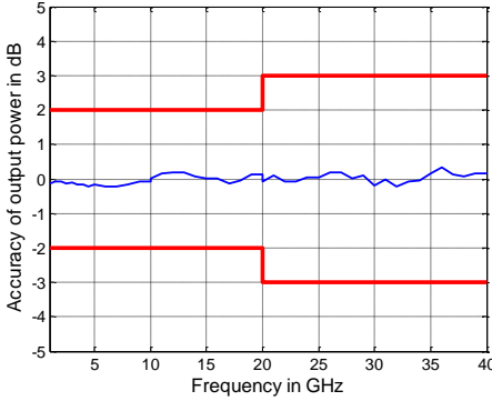
Output power accuracy in dB versus frequency of the R&S ® ZNB40, models .82 and .84
