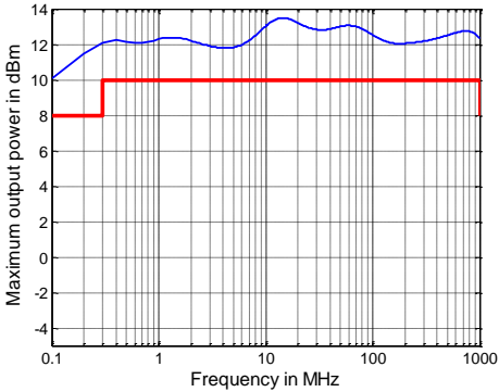
Maximum output power in dBm versus frequency of the R&S ® ZNB40, models .82 and .84
