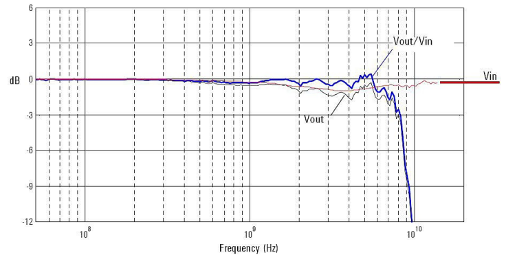
Swept frequency response with a 25- \Omega source
