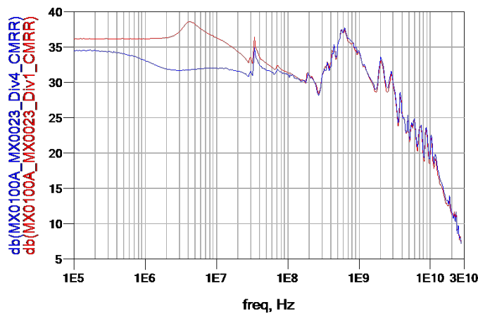
CMRR for the 1:1 (red) and 4:1 (blue) mode.
