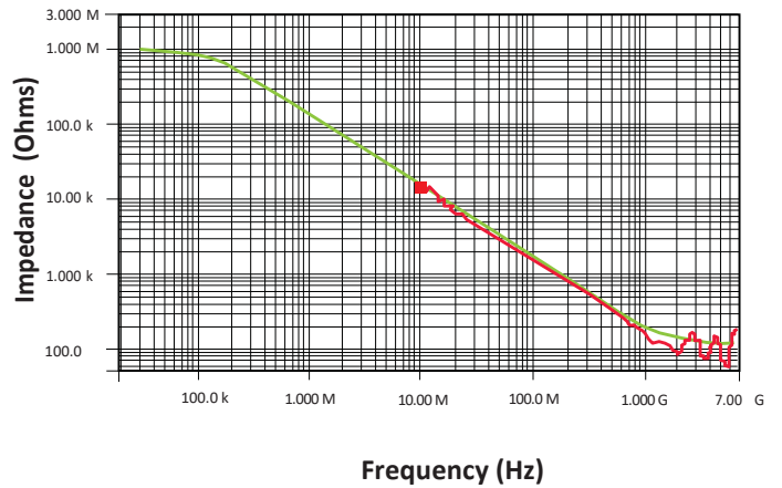
Input impedance over frequency (Red = measured, Green = model)
