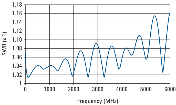
Typical SWR performance
