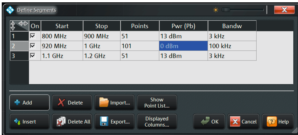
Filter measurement using segmented sweep.
