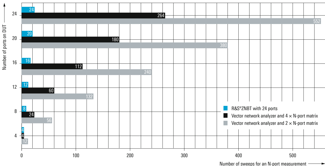
Comparison of measurement time: the R&S®ZNB versus switch matrix based multiport solutions
