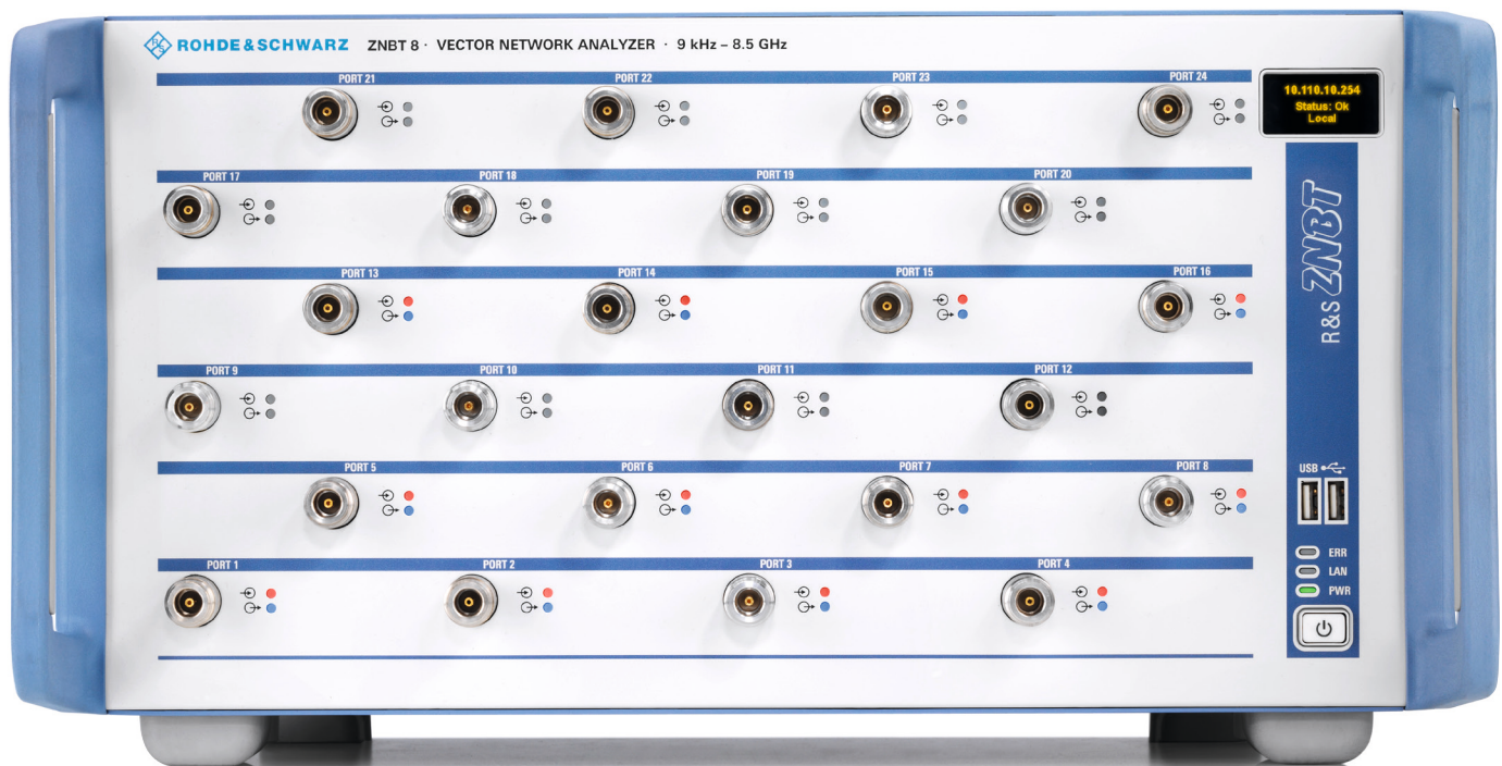
The R&S®ZNB8 with 24 ports.
