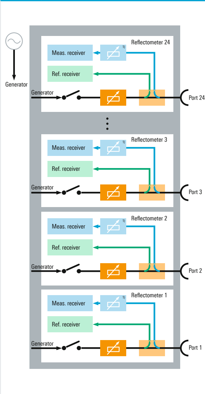
Block diagram of an R&S®ZNBT
