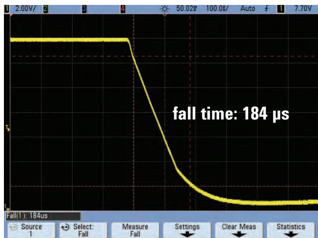
Figure 5. Interrupt pulse fall time measurement of < 200 \mu\text{s}
