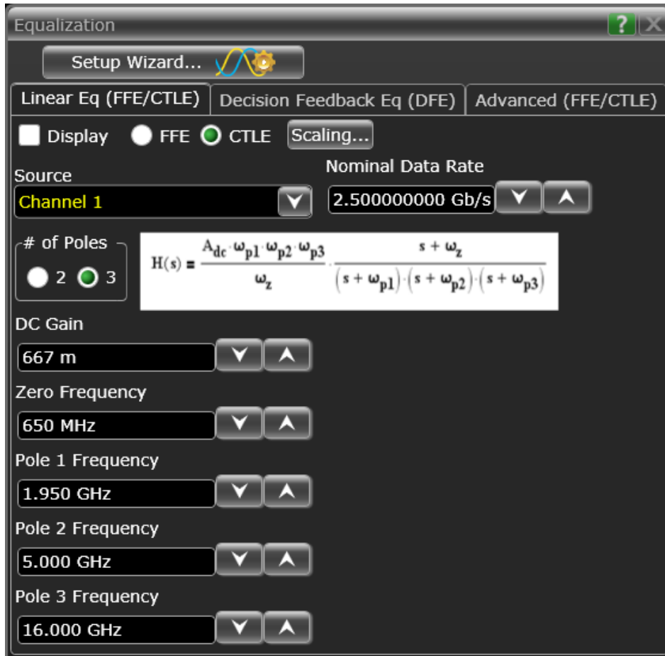
Figure 6. Serial data equalization supports both 2- and 3-pole CTLE.
