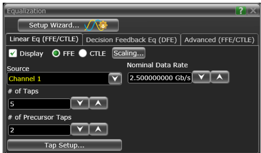
Figure 5. Equalization allows you to choose between FFE, CTLE, and DFE.
