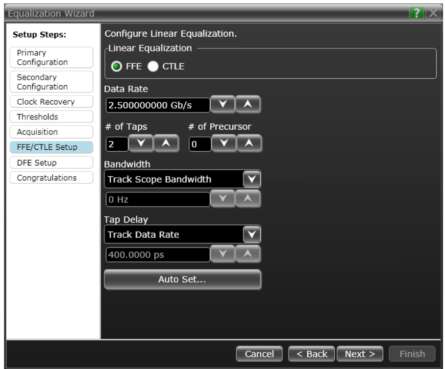
Figure 3. Equalization menu in the equalization wizard.
