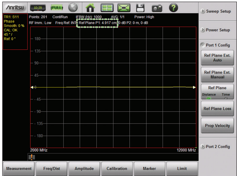
After 1-button Automatic Reference Plane Extension
