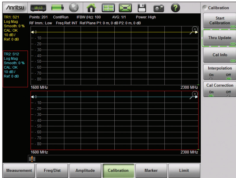
With a simple Through Update, measurement errors caused by the external cable drift is removed
