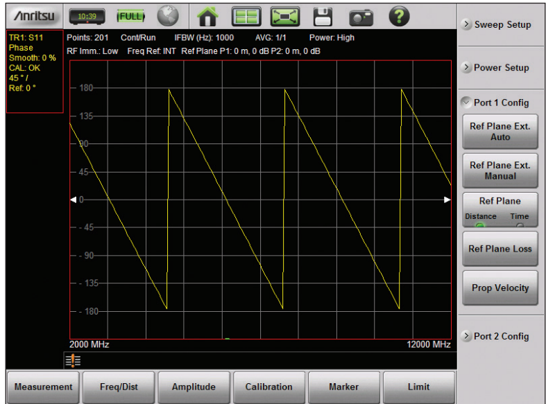
Before 1-button Automatic Reference Plane Extension
