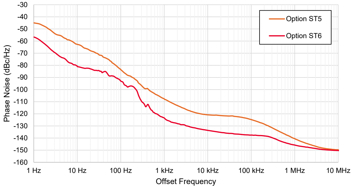
Measured Option ST5 vs. ST6 SSB Phase Noise at 10 GHz
