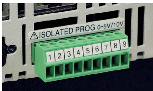
Isolated analog interface (factory option) Voltage control type ISO PROG VOLT CONT PWX OPTION Current control type ISO PROG CURR CONT PWX OPTION
