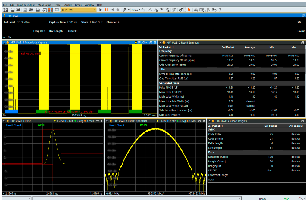
Analysis of a 499.2 MHz wide HRP UWB signal.
