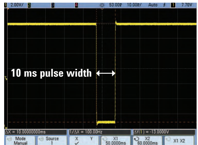
Figure 4. Voltage interrupt pulse generated by N7951A
