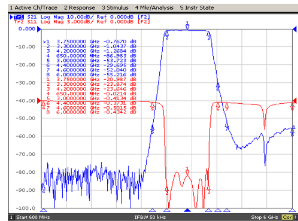
Part Number: G700050616 (3300 to 4200 MHz)
