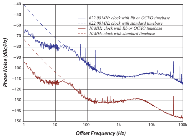
Phase noise for 622.08 MHz and 10 MHz outputs
