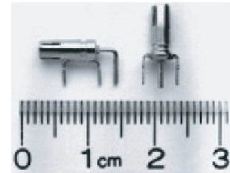
Horizontal and vertical versions of the PC board mini-probe socket make it easy to fit into your target board.
