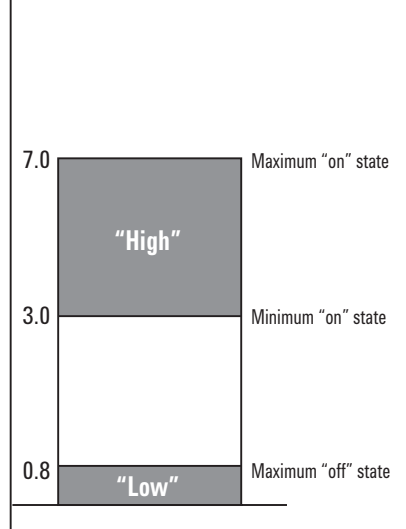
TTL control voltage states (Option T24)
