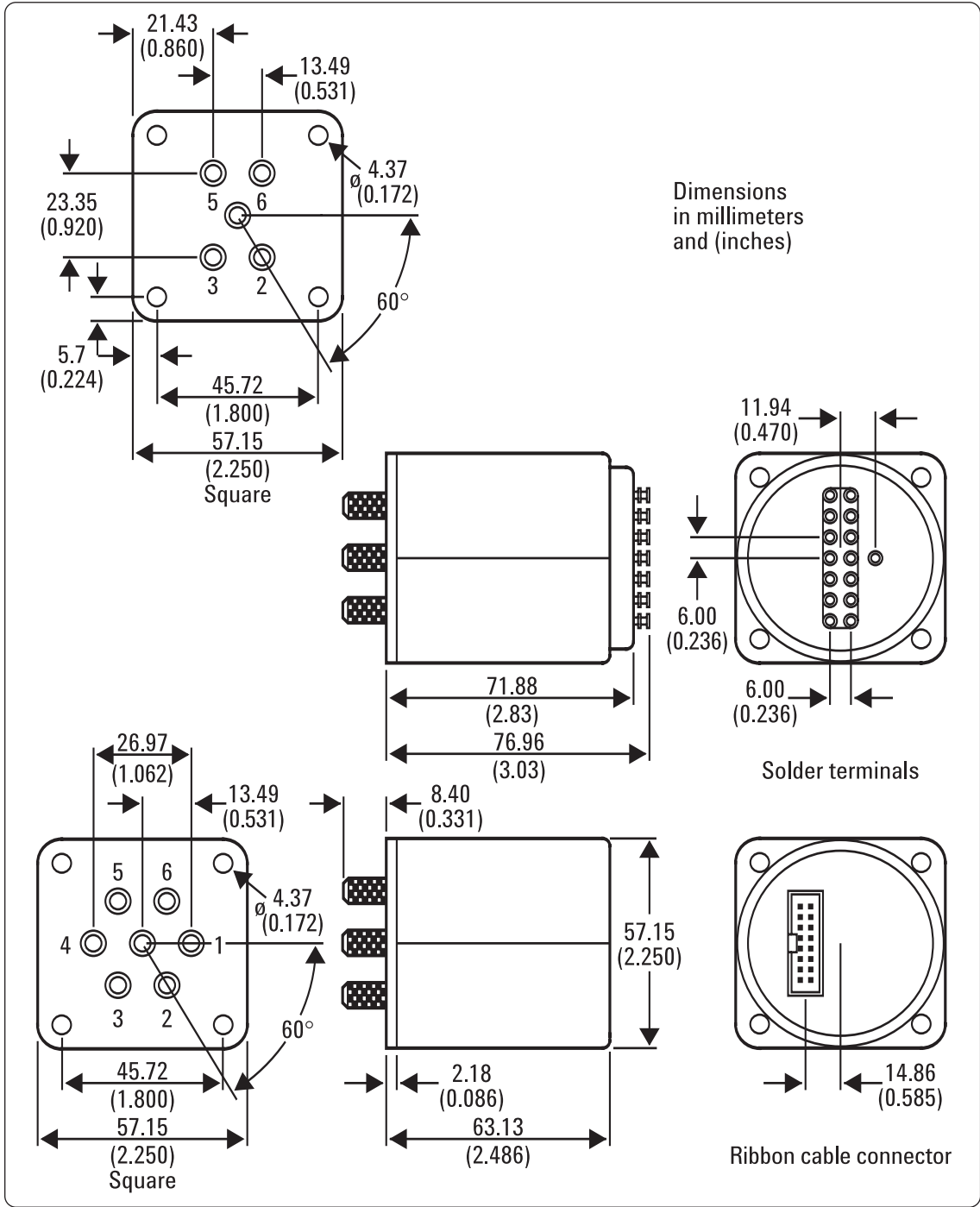
Figure 9. Product outlines
