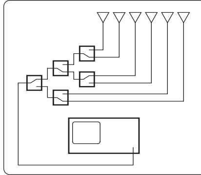
Figure 2. Tree matrix
