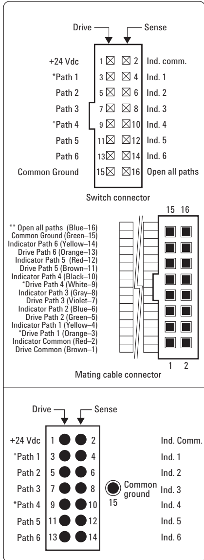
Figure 10. Drive connection diagrams with Option 100
