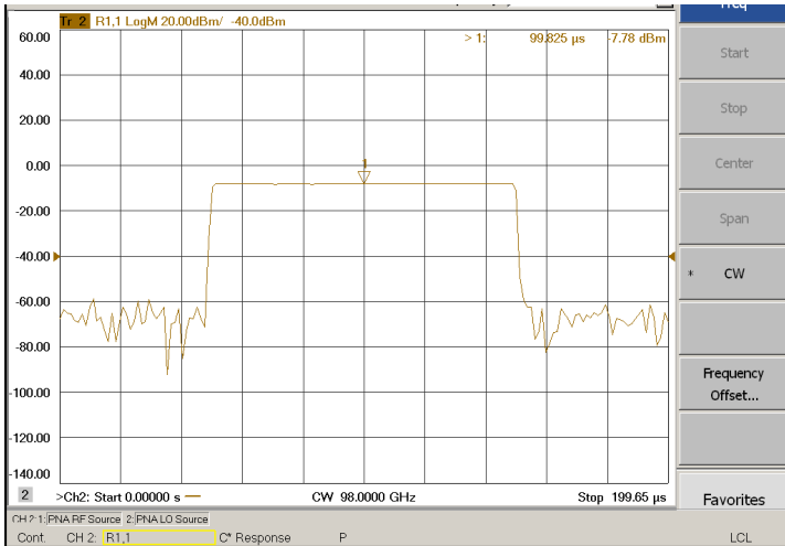
Figure 4. Pulse profile of the calibrated R1 receiver input to an amplifier at 98 GHz
