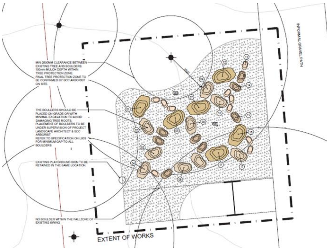
Figure 1: Landscape plan of boulder formation
