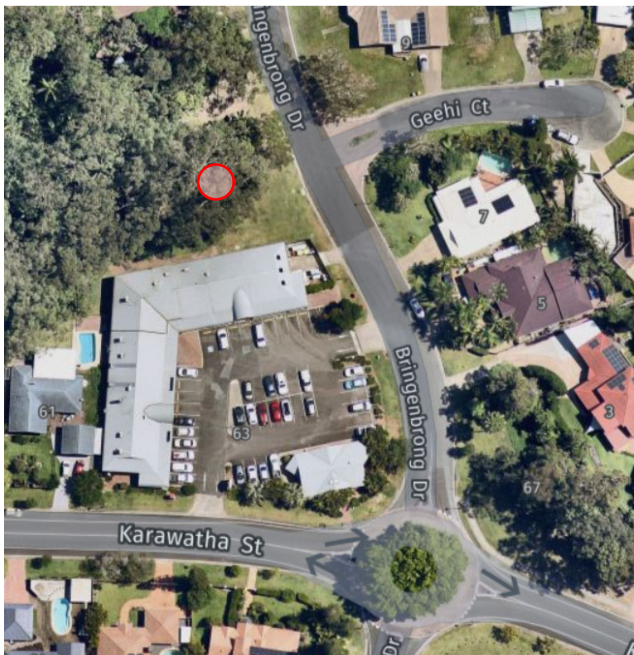
Figure 1: Bringenbrong Drive stormwater headwall replacement location
