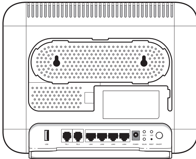
Figure 5-2 XS-2426G-A indoor ONT physical connections (back)
