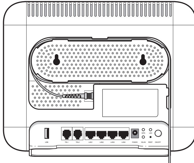
Figure 5-3 XS-2426G-A indoor ONT with fiber optic connector
