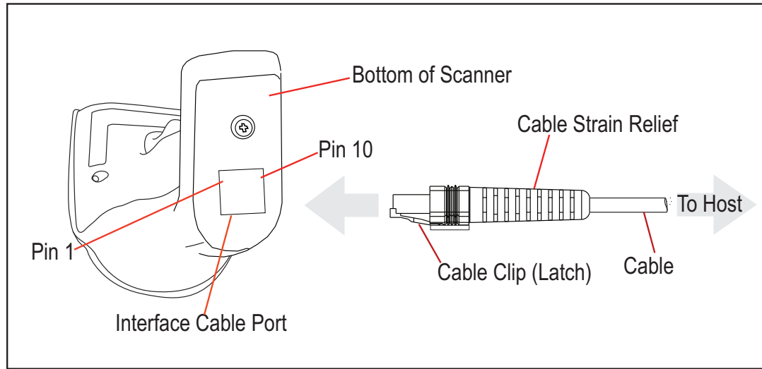
Figure 10. Standard Cable Pinouts: Handheld
