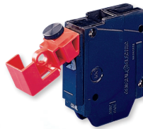
Clamp-On Breaker Lockout Extremely versatile - works on a wide range of single-pole and internal-trip multi-pole breakers. 120/277V # BRA65396 480/600V # BRA65397
