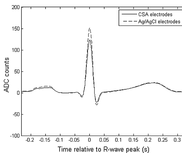
FIGURE 5. Averaged ensembles of ECG signals acquired using Ag/AgCl and carbon/salt/adhesive electrodes, for the same subject.
