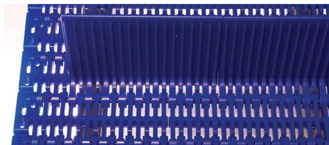
S800 Flush Grid belting features 27% open area.
