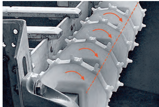
Figure 40: Align sprocket teeth
