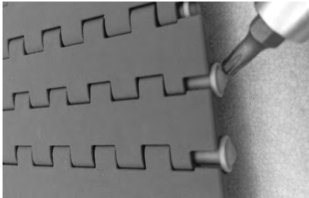
Figure 133: Push rod past retention feature
