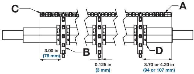
A Belt B Sprocket C Inside edge of belt D Split heavy-duty retainer ring Figure 366: Belt width of 16 in (407 mm) and less
