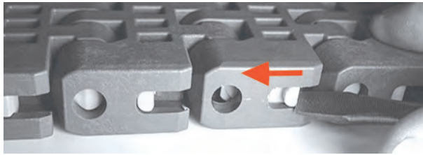
Figure 159: Close Slidelox
