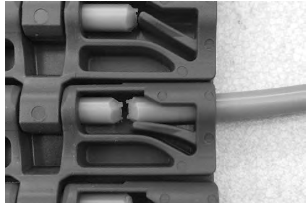
Figure 130: Push retention feature open
