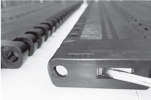
Figure 215: Close the Slidelox
