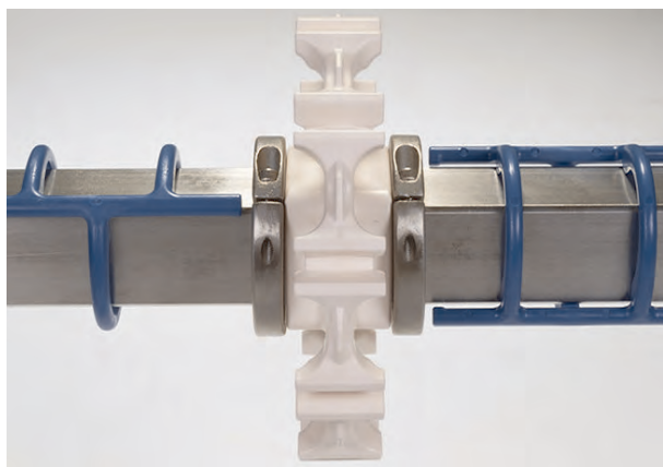
Figure 11: Place retainer ring at centerline
