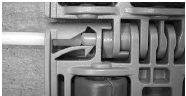
Figure 223: Push rod past retention feature
