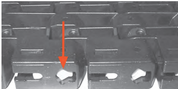
Figure 185: Open Slidelox
