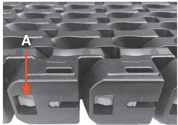
Figure 201: Close Slidelox
