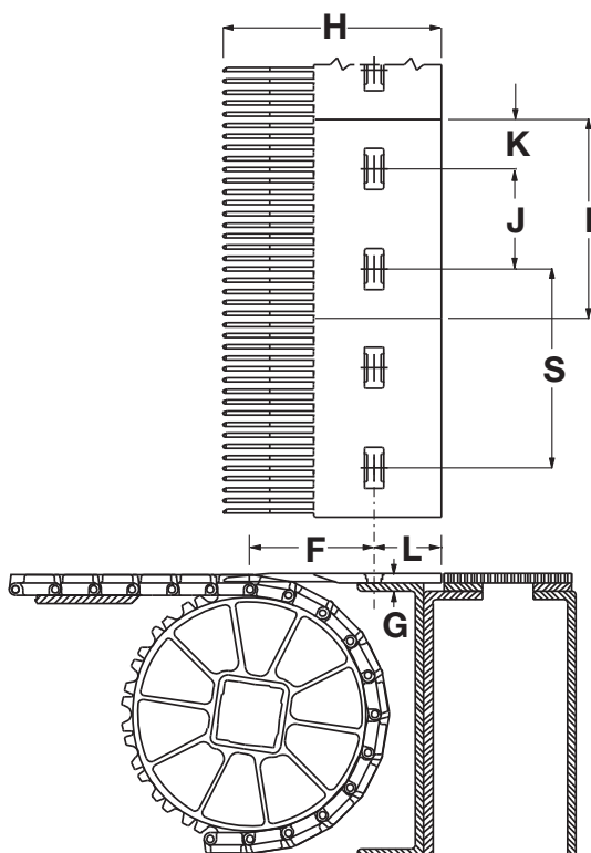
Figure 25: Finger transfer plates location
