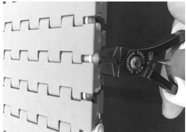
Figure 135: Cut rod head
