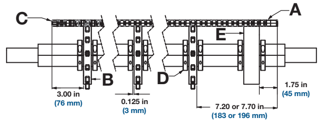
A Belt B Sprocket C Inside edge of belt D Split heavy-duty retainer ring E Support wheel Figure 364: Belt width of 16 in (407 mm) to 24 in (610 mm)
