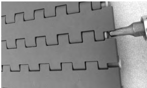
Figure 134: Cut opposite end of rod
