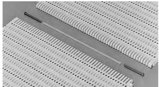
Figure 31: Abrasion resistant rod and rodlets
