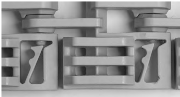
Figure 87: Ensure rod is past retention feature
