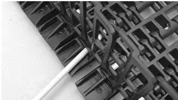
Figure 369: Insert rod through hinges
