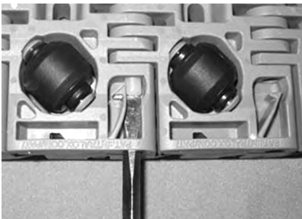
Figure 232: Push rod past retention feature
