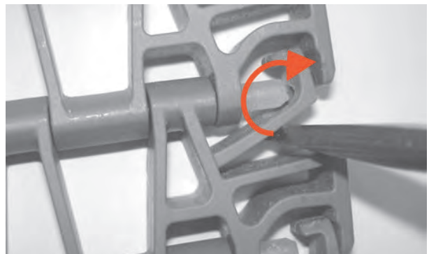
Figure 254: Rotate screwdriver to hold retention feature open
