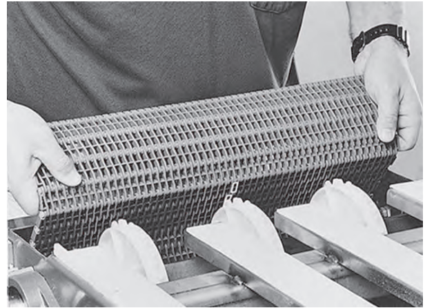
Figure 18: Wrap belt around drive sprockets
