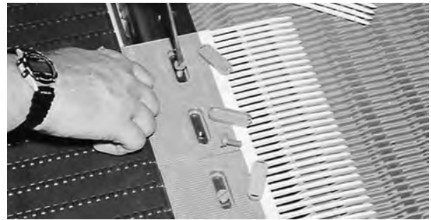
Figure 24: Install finger transfer plates using Intralox plastic bolts
