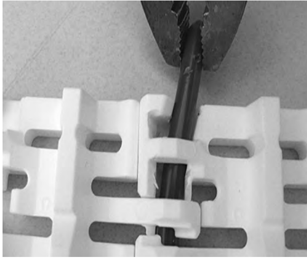
Figure 84: Pull rod from belt
