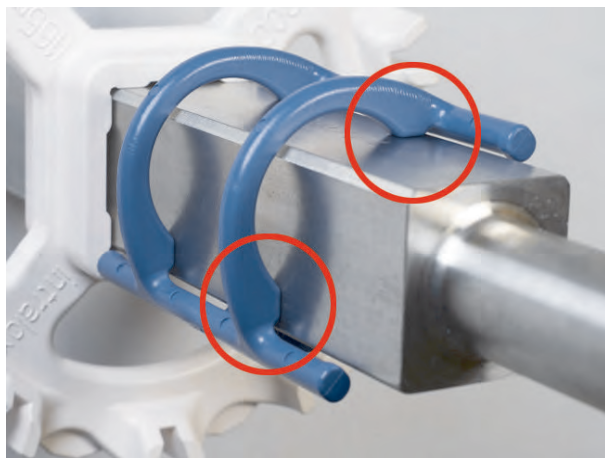
Figure 9: Ensure spacer is flat against shaft
