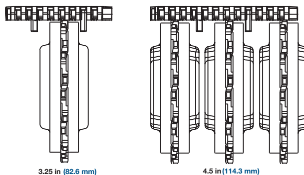
Figure 167: Sprocket tracking tabs
