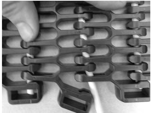
Figure 329: Align hinges
