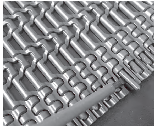
Figure 62: Lift rod over retention feature
