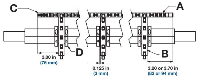
A Belt B Sprocket C Inside edge of belt D Split heavy-duty retainer ring Figure 363: Belt width of 16 in (407 mm) and less
