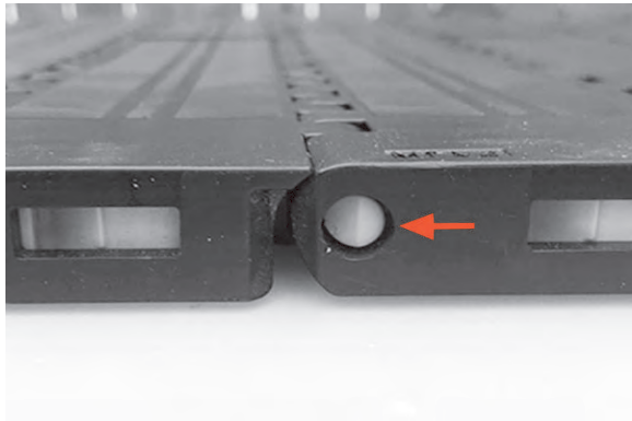
Figure 209: Slidelox in closed position
