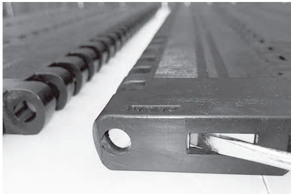
Figure 210: Use screwdriver to close Slidelox
