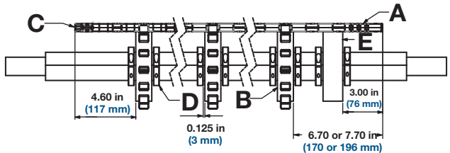
Figure 352: Belt width of 16 in (407 mm) and less
