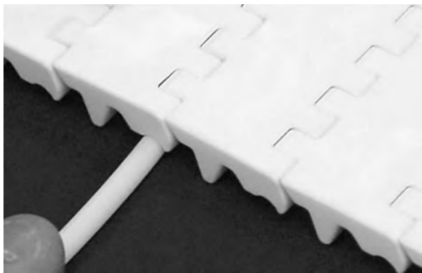
Figure 174: Insert rod through hinges
