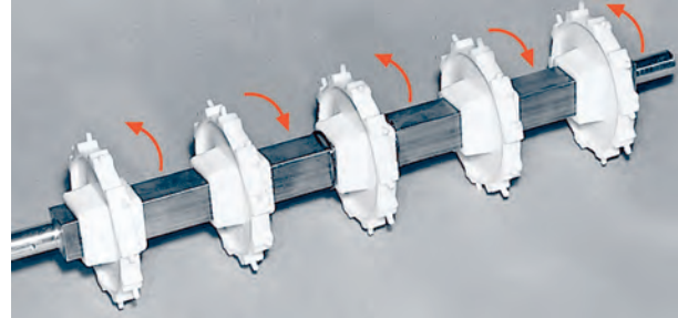
Figure 41: Reverse every other sprocket
