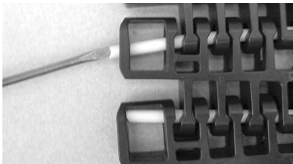
Figure 360: Push rod past retention feature
