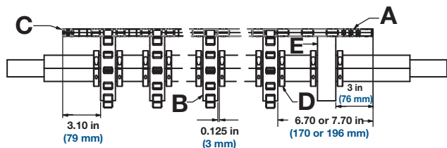
Figure 346: Belt width of 24 in (610 mm) and less
