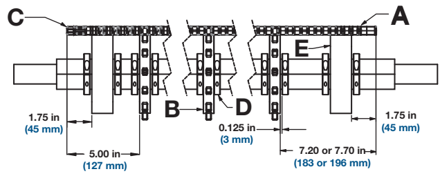
A Belt B Sprocket C Inside edge of belt D Split heavy-duty retainer ring E Support wheel Figure 365: Belt width of 24 in (610 mm) and more
