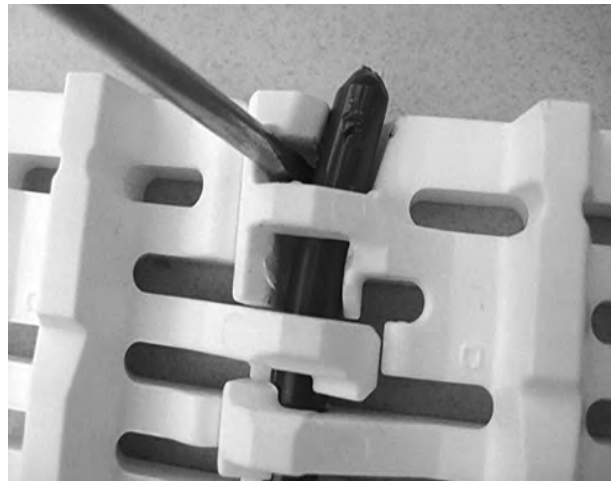
Figure 83: Lift rod past retention feature
