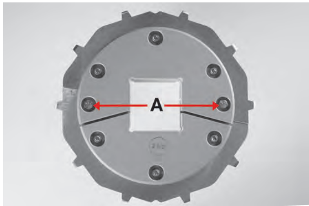
Figure 6: S7000 split sprocket
