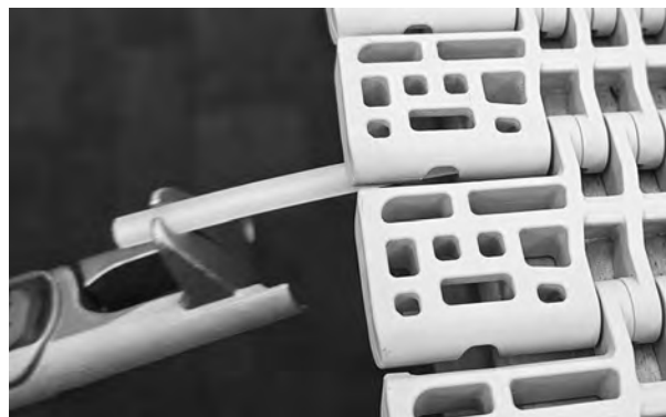
Figure 127: Pull rod down and out of belt
