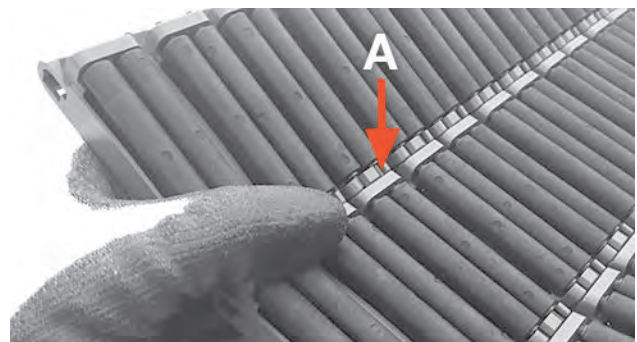
A Pinch point Figure 246: Pinch points occur if belt backbends
