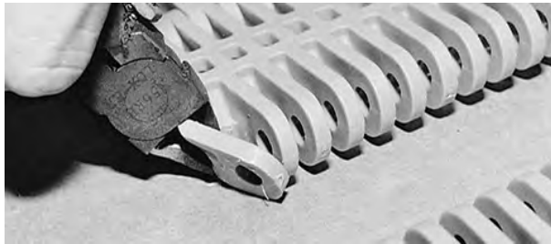
Figure 52: Cut outermost link
