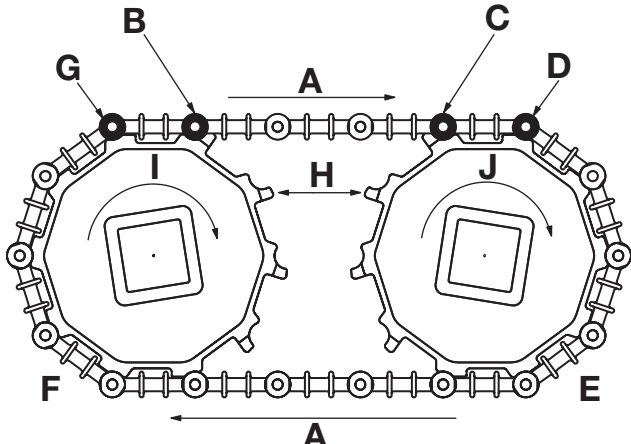
Figure 40: Align sprocket teeth
