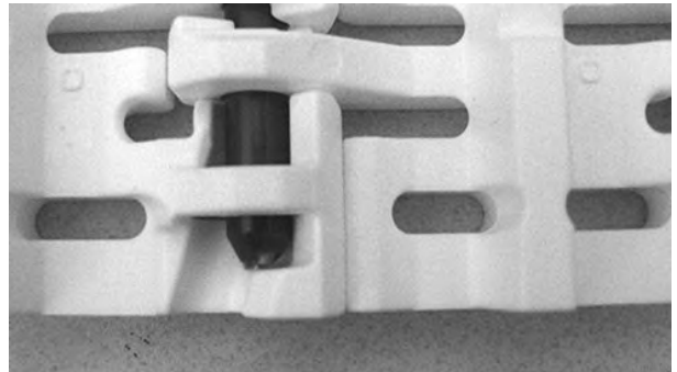
Figure 82: Ensure rod is fully inserted
