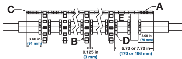
Figure 349: Belt width of 16 in (407 mm) and less
