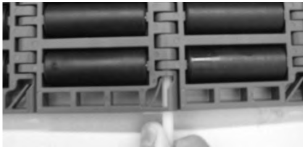
Figure 237: Insert rod through hinges
