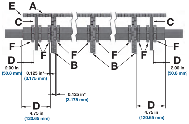
Figure 325: S2600-1.0 >= 26 in (660.4 mm)
