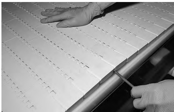
Figure 90: Push rod through the hinges until fully seated
