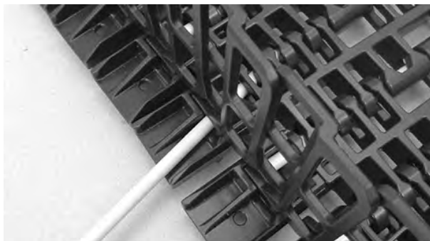
Figure 355: Insert rod through hinges
