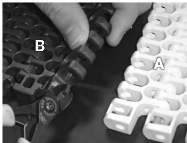
Figure 299: Trim rod guides from old design module (B)
