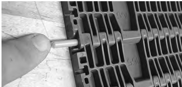
Figure 271: Insert rod
