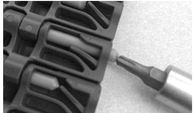
Figure 129: Push rod past retention feature
