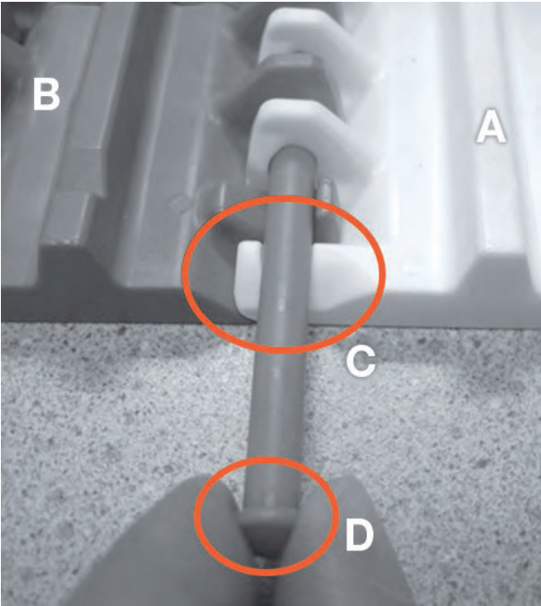
A Updated design B Original design C New rod retention geometry D Rod head
