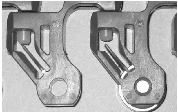
Figure 284: Ensure rod is past retention feature
