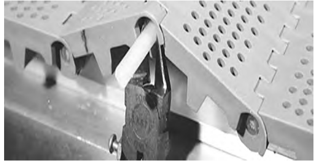
Figure 66: Cut rod flush with belt edge
