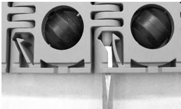
Figure 56: Push rod past retention feature
