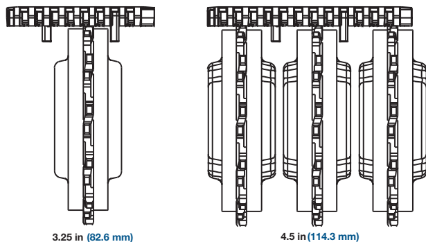
Figure 111: Sprocket tracking tabs
