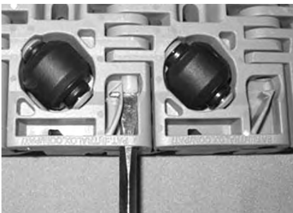
Figure 226: Push rod past retention feature
