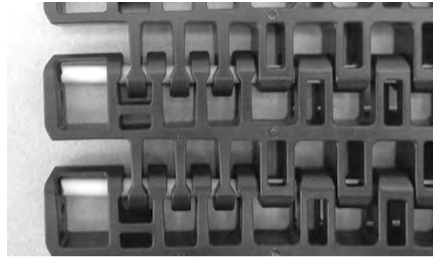
Figure 361: Ensure rod is past retention feature
