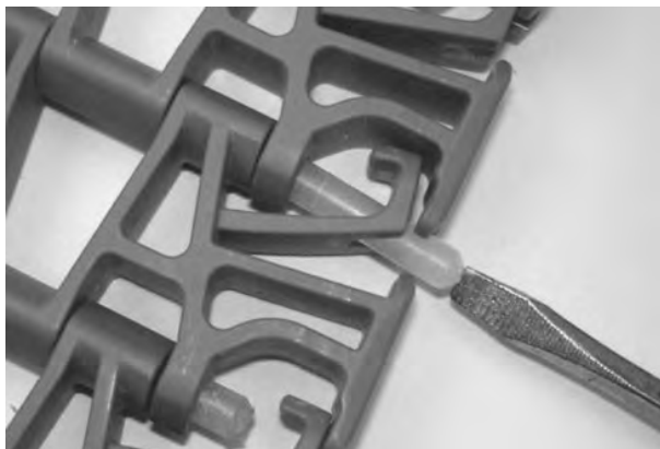
Figure 252: Push rod past retention feature
