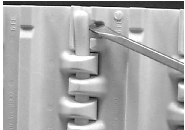
Figure 207: Lift rod over retention feature
