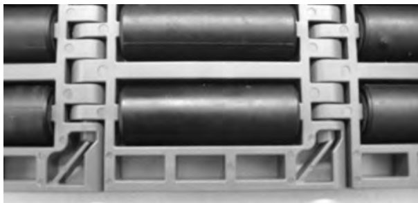
Figure 239: Ensure rod is past retention feature
