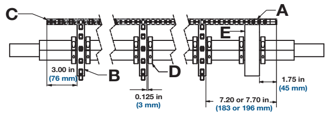
A Belt B Sprocket C Inside edge of belt D Split heavy-duty retainer ring E Support wheel Figure 367: Belt width of 16 in (407 mm) to 24 in (610 mm)
