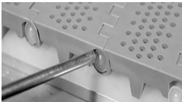
Figure 65: Ensure rod head is past snap-lock
