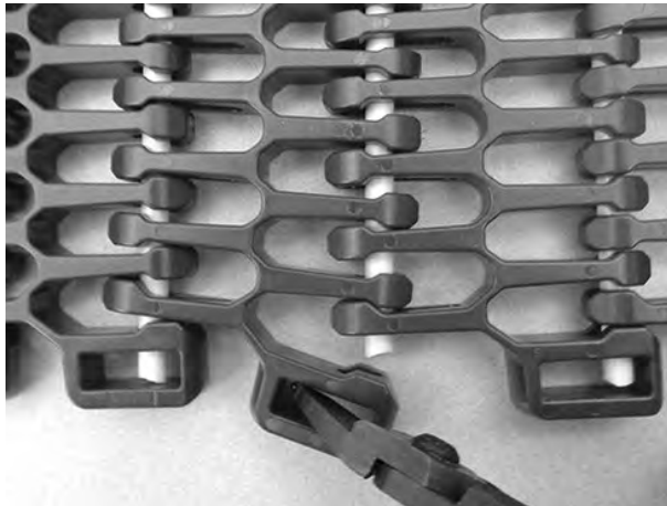
Figure 332: Flex flush edge of module
