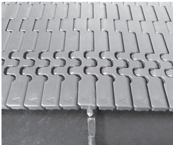
Figure 60: Push rod past retention feature
