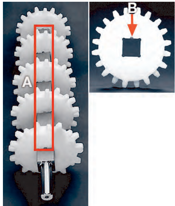
A Notches aligned B Sprocket alignment notches Figure 3: Ensure sprocket alignment notches are aligned
