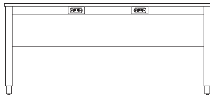
Communal Table at Breakfast Room (K/D) 3176A20B20 90 x 34 x 40 #211
