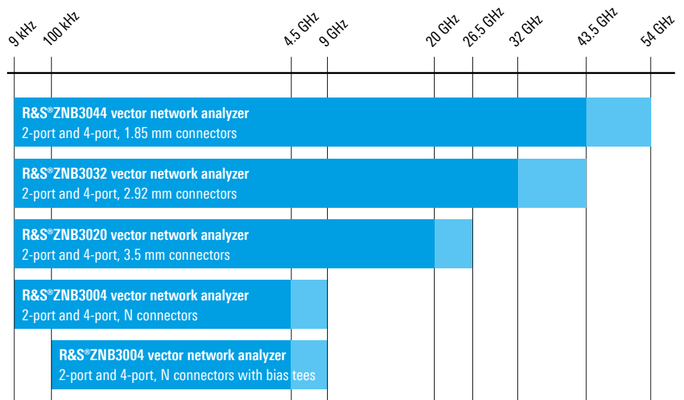
R&S®ZNB3000 models
