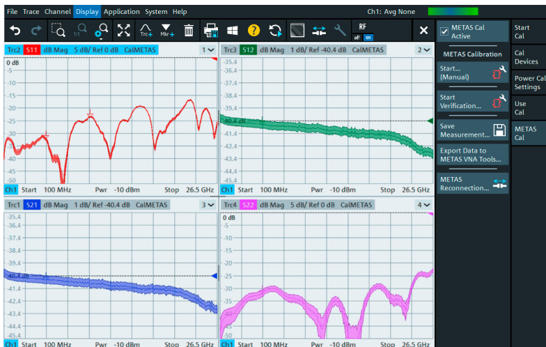
Real-time S-parameter measurements with uncertainty bands
