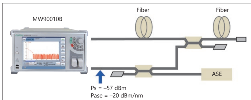
Measurement Setup for Dynamic Range
